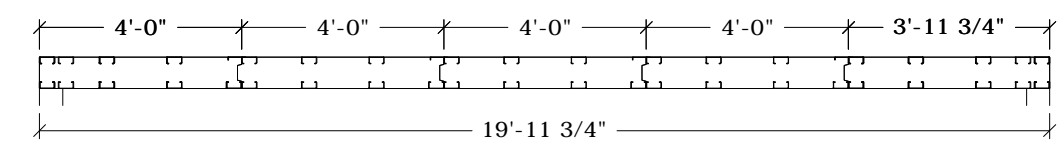
Roof 2 7 1/2" PANELS 362S162-33 @ 16" O.C. (1.5PCF EPS DENSITY)
