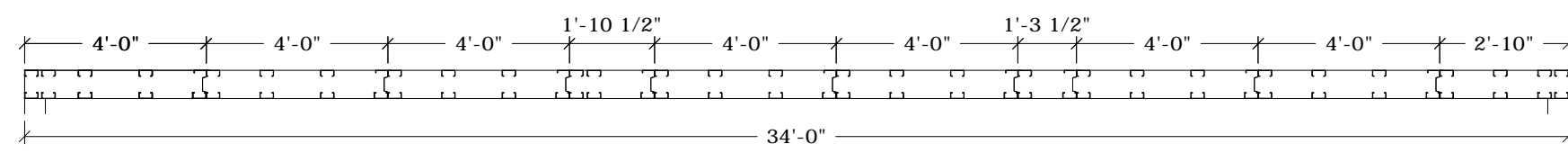
Roof 1 7 1/2" PANELS 362S162-33 @ 16" O.C. (1.5PCF EPS DENSITY)
