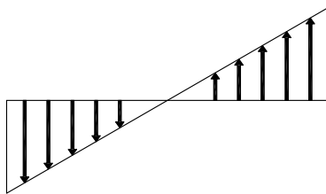
STANDARD SHEAR WALL PANEL SHEAR RACKING STRUCTURAL FRAME
